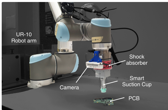
Fig. 7: Experimental setup for the pick and place test on the tabletop system.
